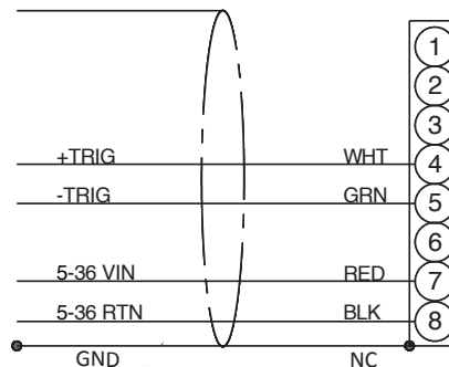
MPS FLYING LEADS CABLE CONNECTIONS
